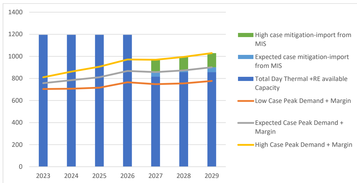
Figure 12 Resource Adequacy – DPS
