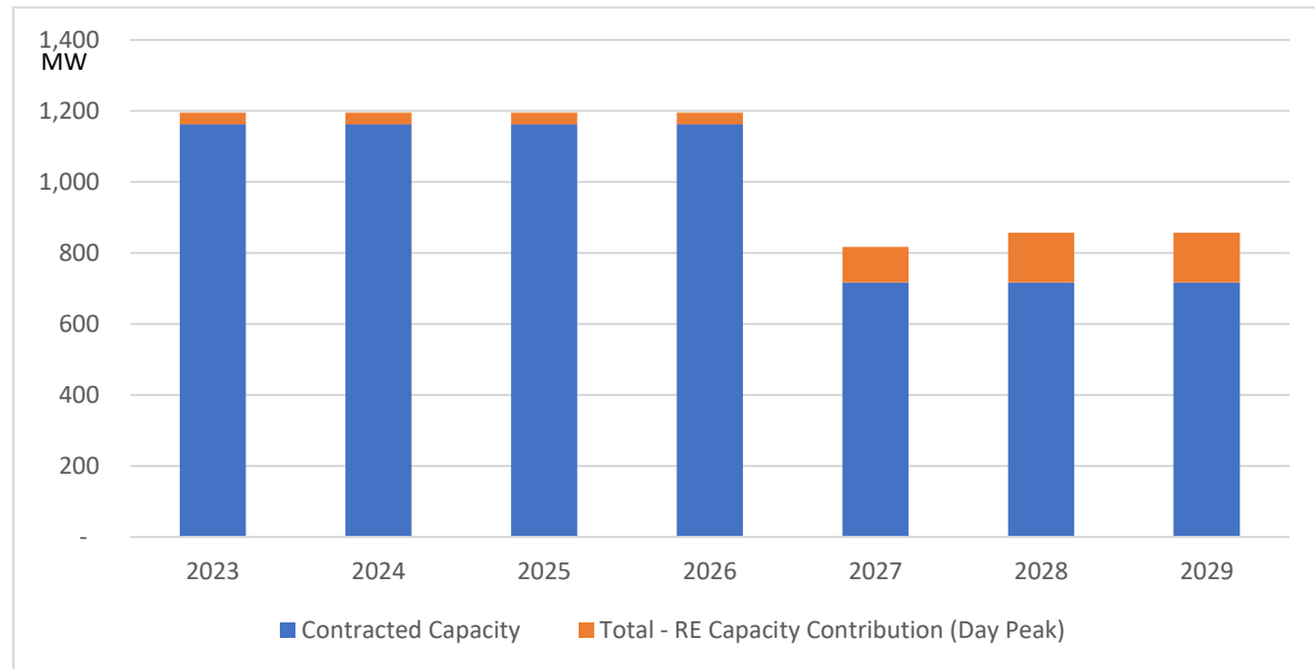
Figure 11 Capacity Contributions from Generation Resources During the Day Peak– DPS
