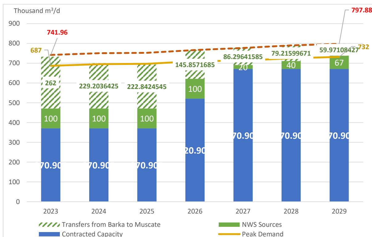
Figure 20 Resource Adequacy and Development Plan – Muscat Zone
