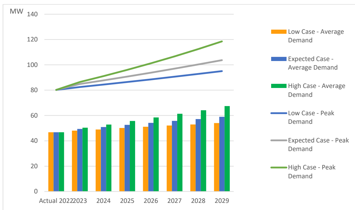
Figure 13 Electricity Demand Projections – Musandam Power System
