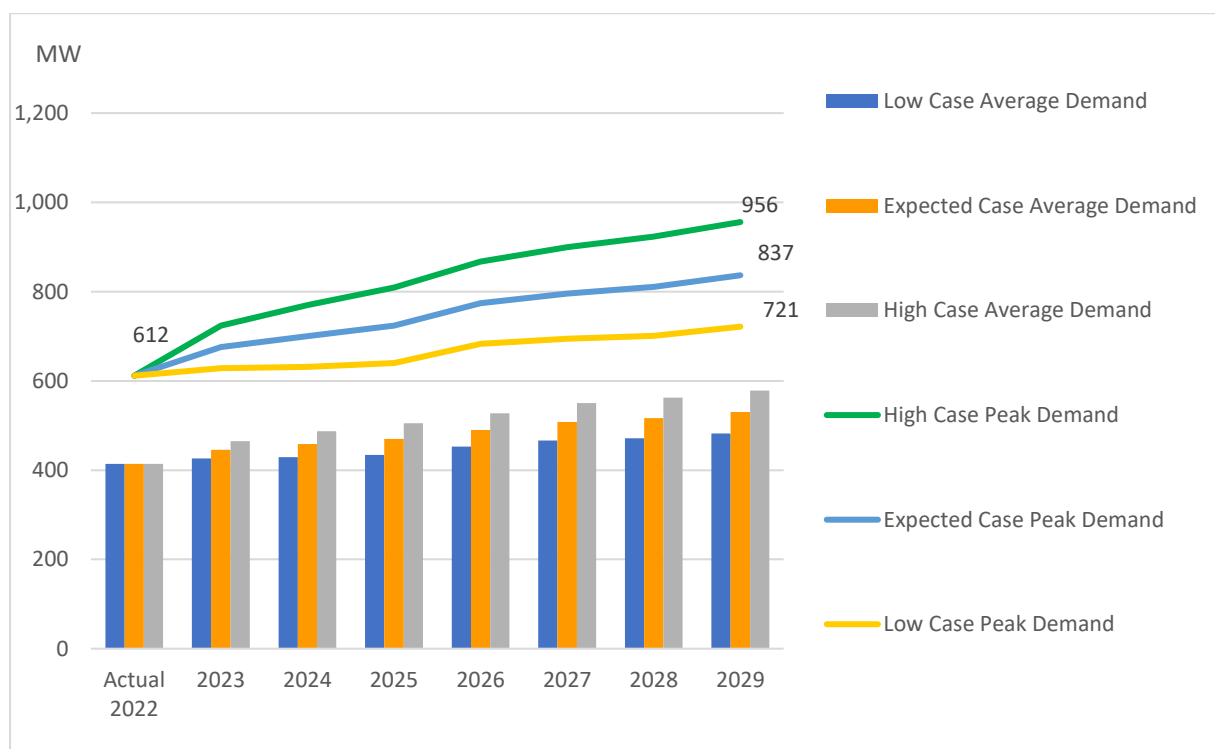
Figure 10 Electricity Demand Projections – DPS
