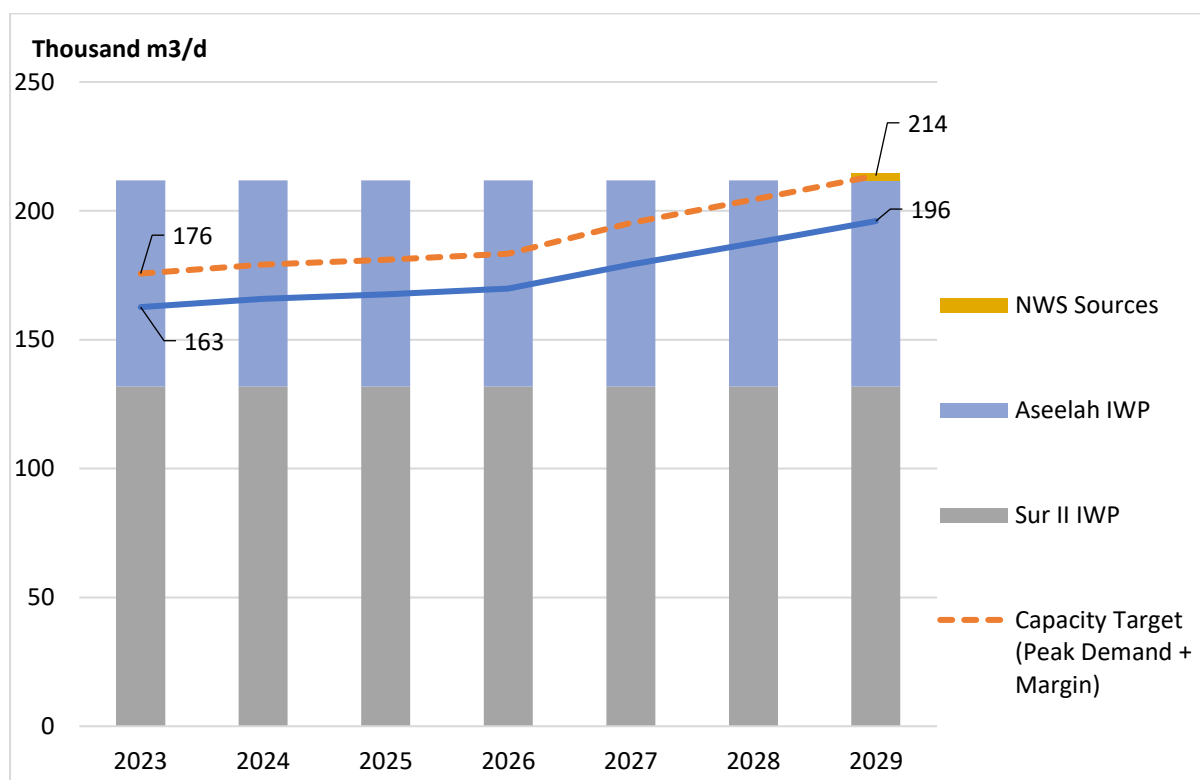
Figure 24 Resource Adequacy and Development Plan – Sharqiyah Zone
