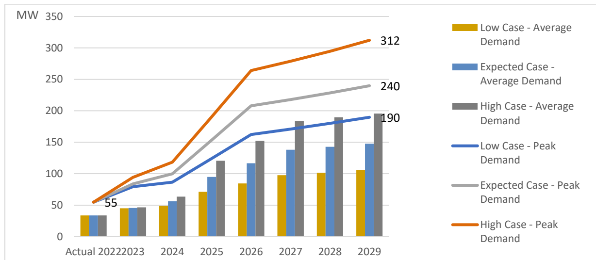
Figure 3 Electricity Demand Projections – Ad Duqm Power System
