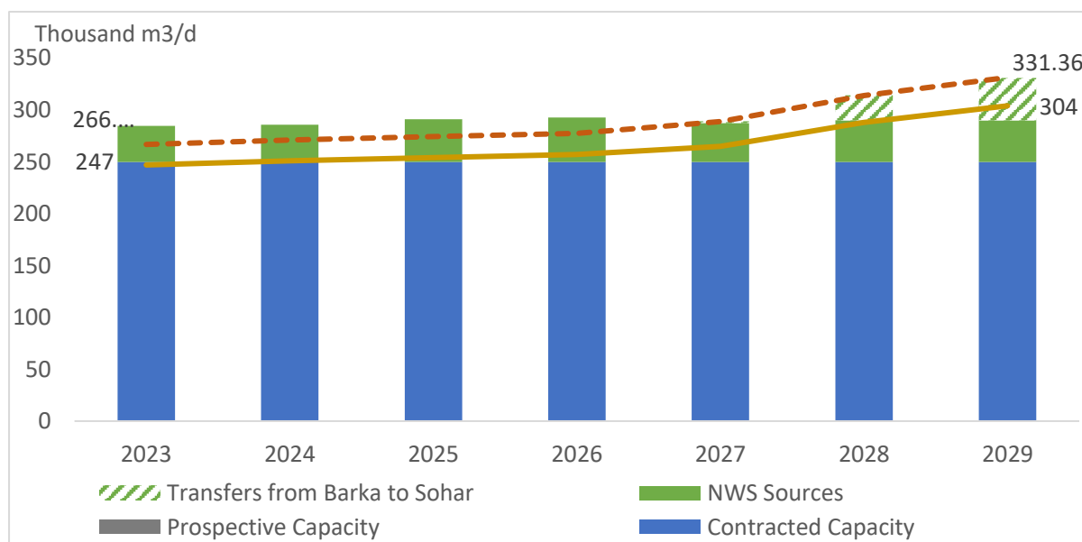
Figure 22 Resource Adequacy and Development Plan – Sohar Zone
