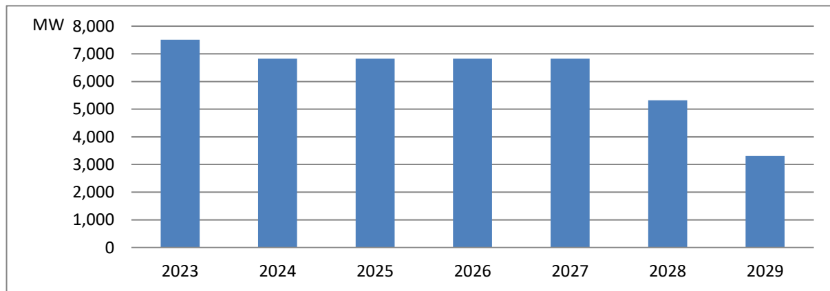
Figure 4 Contracted Generation Capacity – MIS
