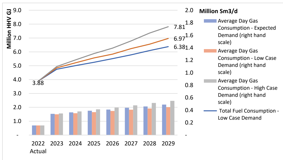
Figure 18 Projected Fuel Requirements – Musandam Power System
