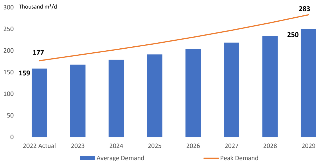
Figure 25 Water Demand Projections – Dhofar Zone
