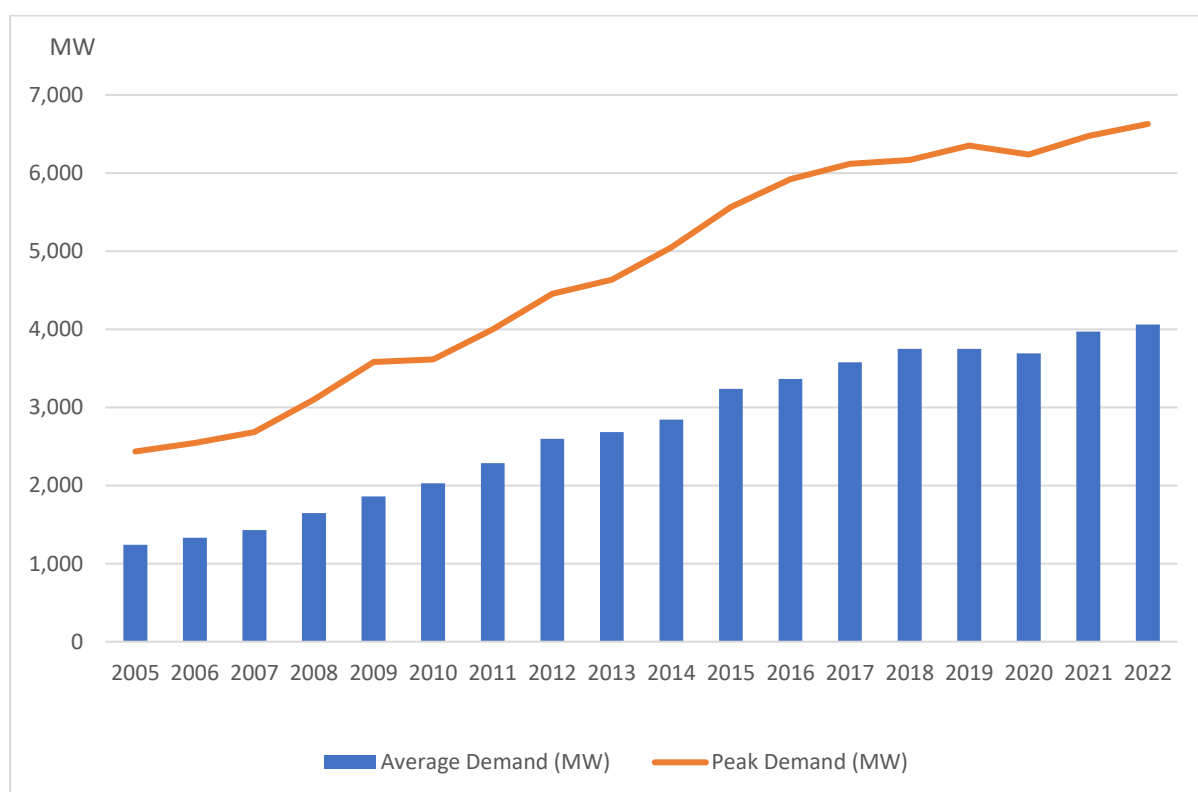
Figure 1 MIS Historical Electricity Demand – MIS
