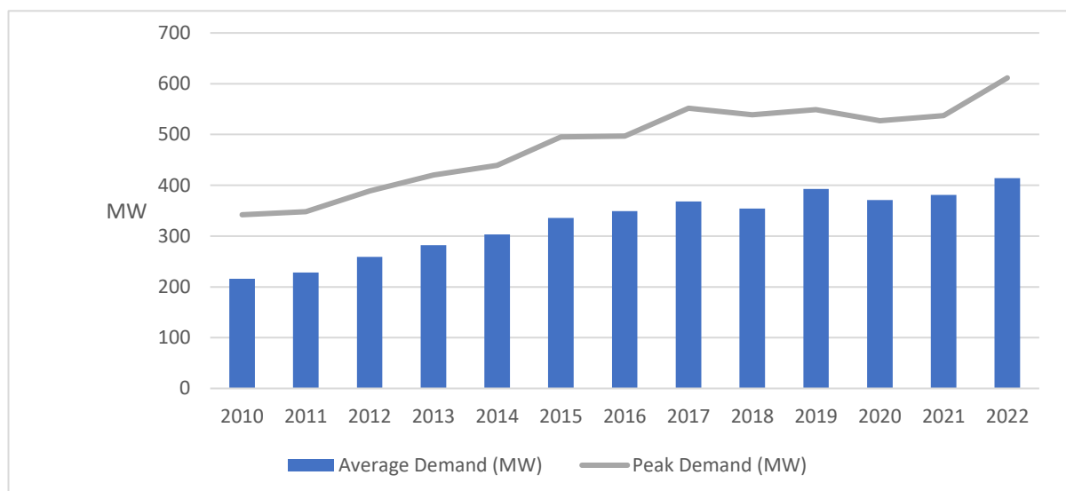
Figure 9 Historical Electricity Demand – DPS
