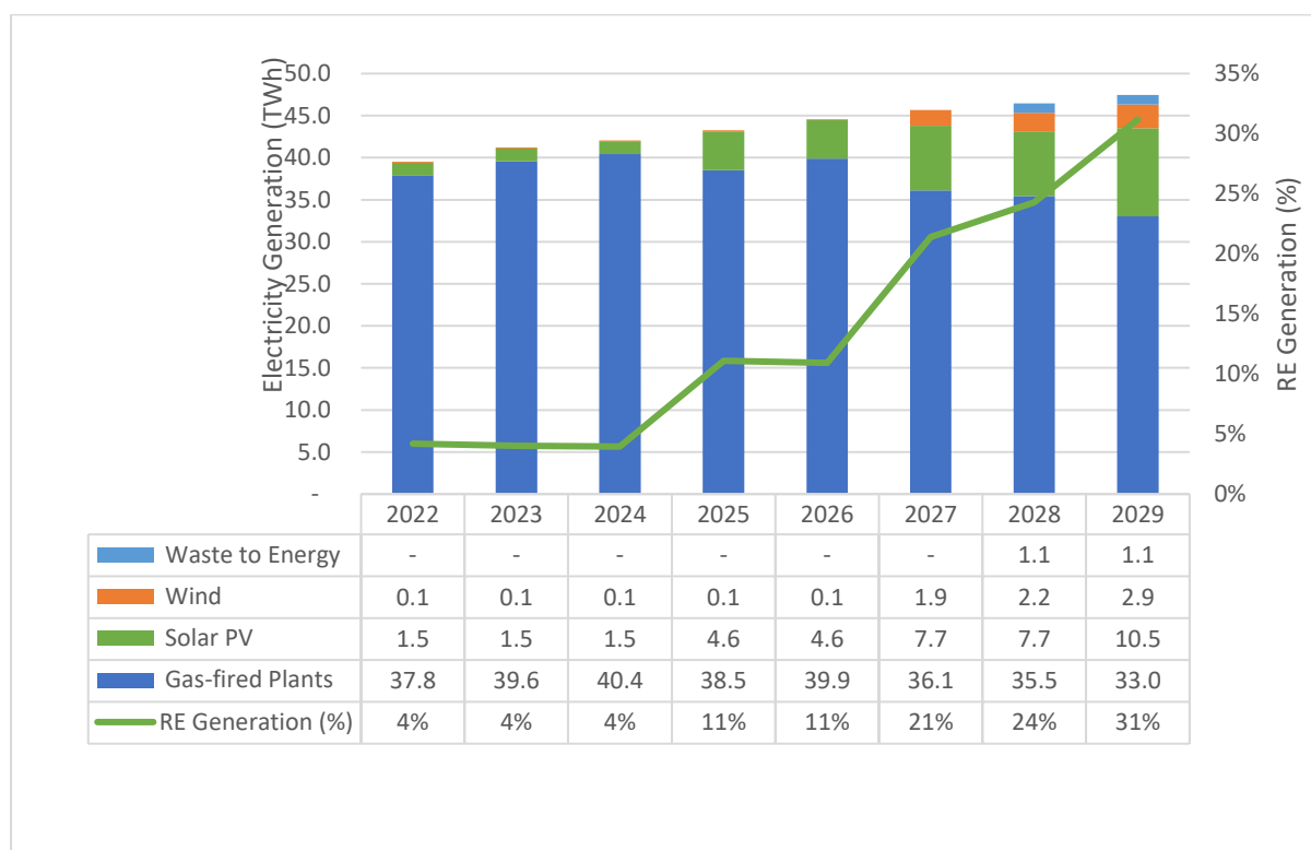
Figure 15 Fuel Shares in Electricity Generation
