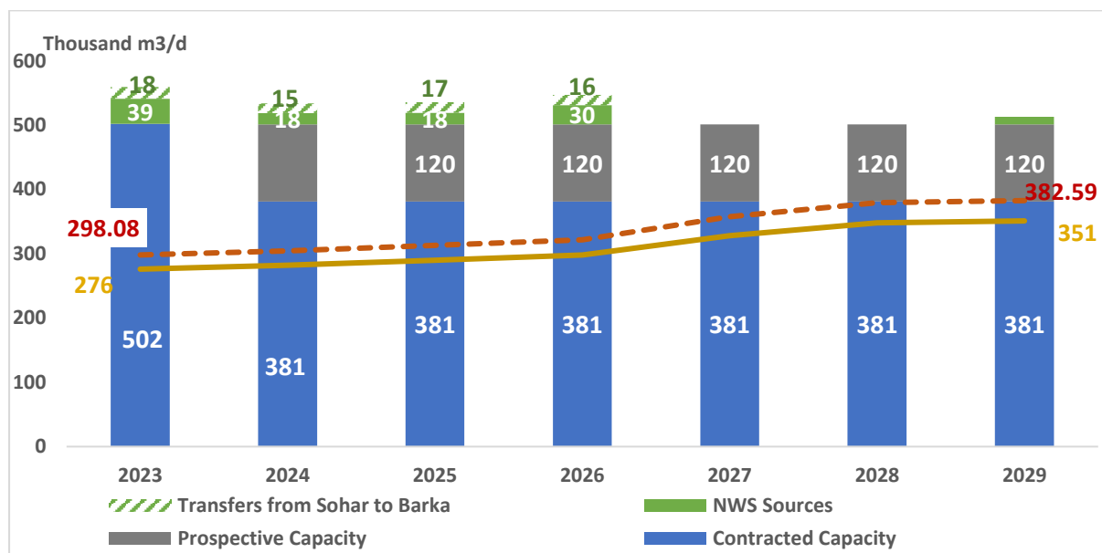
Figure 21 Resource Adequacy and Development Plan – Barka Zone
