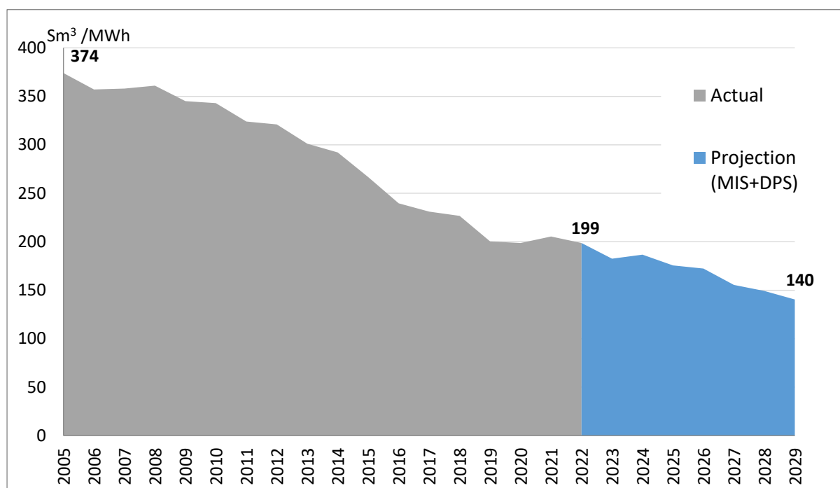
Figure 16 Gas Required per Unit of Electricity Generation – MIS + DPS
